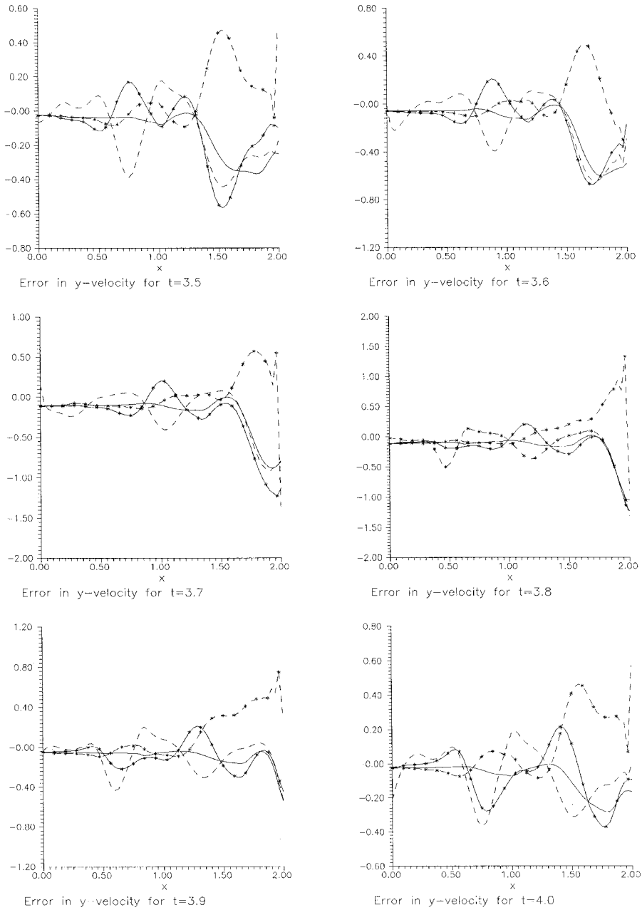
Figure 17. Error in u_2 for y=0.5 , where * , b.c. with U^0 ; \times , b.c. with U^1 ; —, b.c. with U^2 ; ---, HS b.c.
