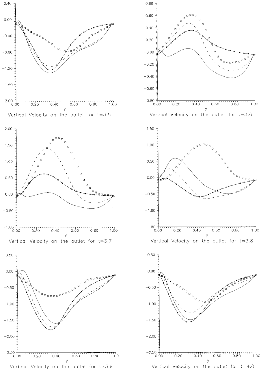
Figure 19. u_2 profile on the outlet ( x=2 ), where \square , exact; - * - , b.c. with U^0 ; - \times - , b.c. with U^1 ; - , b.c. with U^2 ; - - - , HS b.c.
