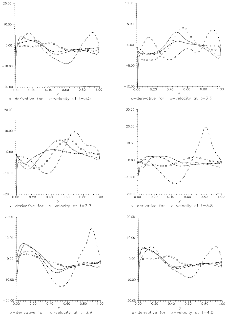
Figure 20. \partial u_1/\partial x on the outlet ( x = 2 ), where \square , exact; - * - , b.c. with U^0 ; - \times - , b.c. with U^1 ; - , b.c. with U^2 ; - \cdot - , HS b.c.
